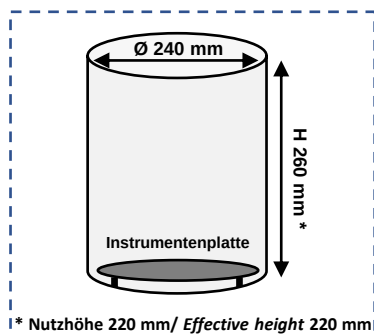
Kammer Chamber
